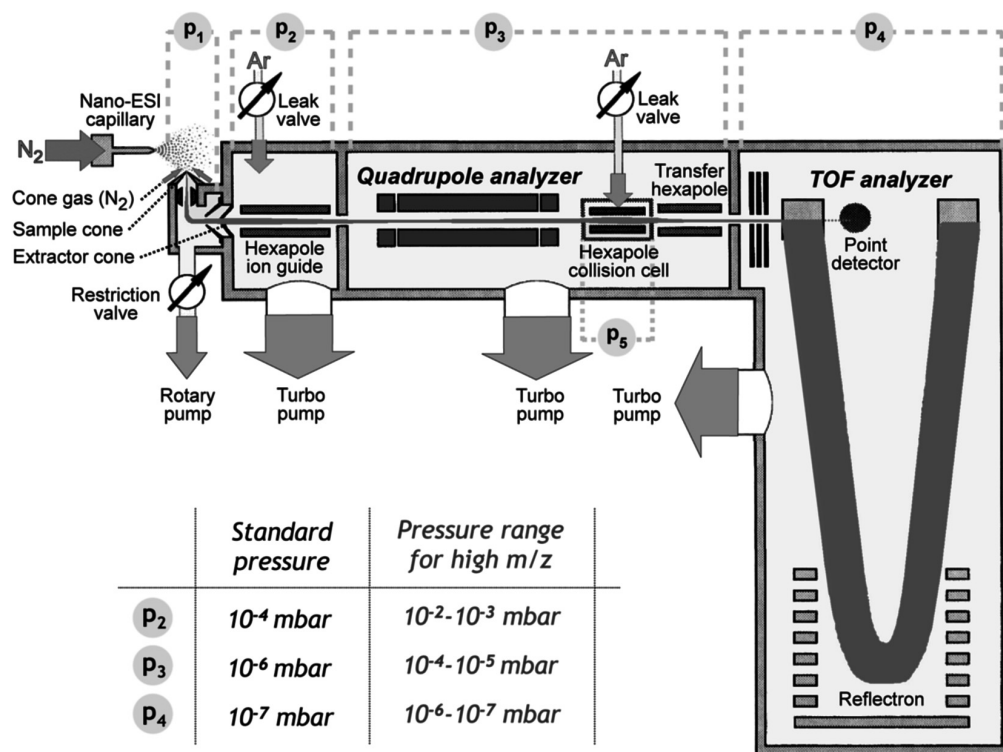
FIGURE 1. Diagram showing the different pressure regimes in the modified Q-TOF 2 mass spectrometer (Micromass UK) (Sobott et al. 2002). Reducing the efficiency of pumping in the source and intermediate pressure regions, as well as admitting a collision gas to the collision cell, improves the transmission of high-mass species through the instrument.
