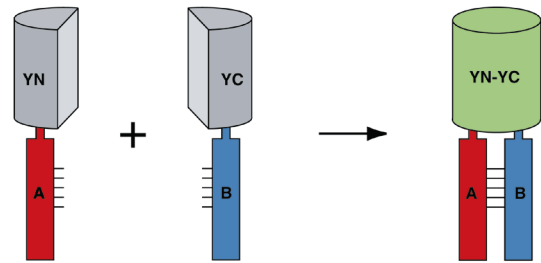
FIGURE 1. Schematic representation of the principle of the BiFC assay. Two nonfluorescent fragments (YN and YC) of the yellow fluorescent protein (YFP) are fused to putative interaction partners (A and B). The association of the interaction partners allows formation of a bimolecular fluorescent complex.
